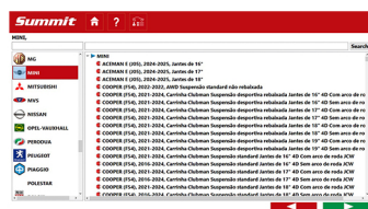
Model selection
